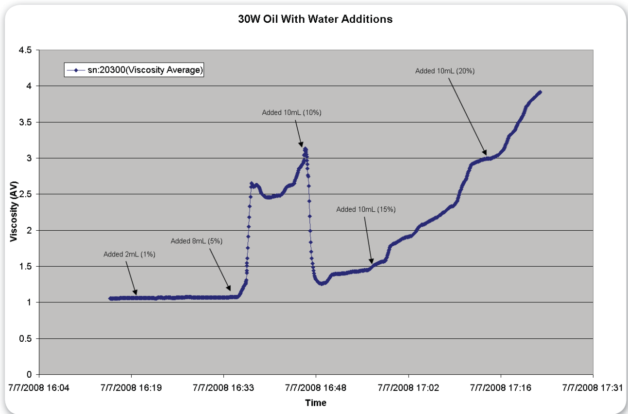
Figure 3 –ViSmart™ viscosity sensor tracking viscosity changes due to water contamination.
