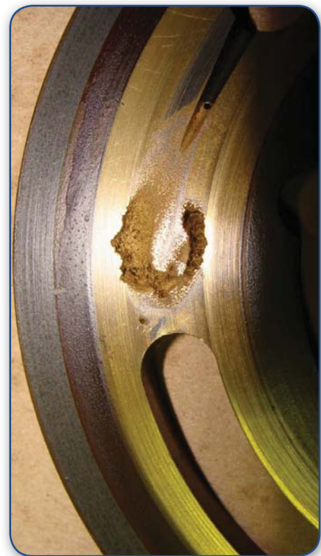
Figure 1 – Cavitation damage on a valve plate for an axial piston hydraulic pump.
