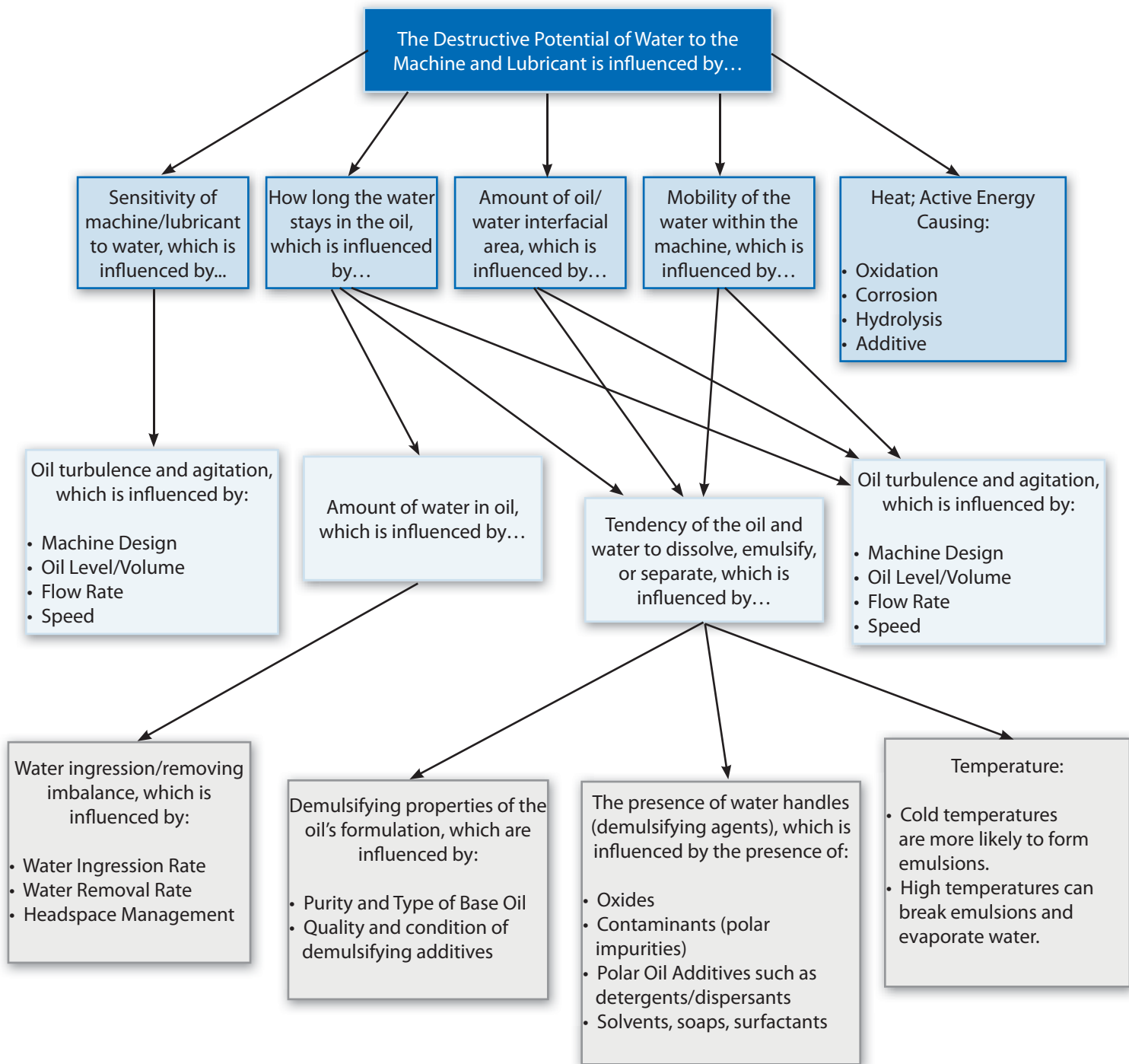
Figure 2: The effect of water contamination on machinery. Chart Reproduced from "The Hazards of Water Handles" by Jim Fitch, Practicing Oil Analysis Magazine. November 2004
