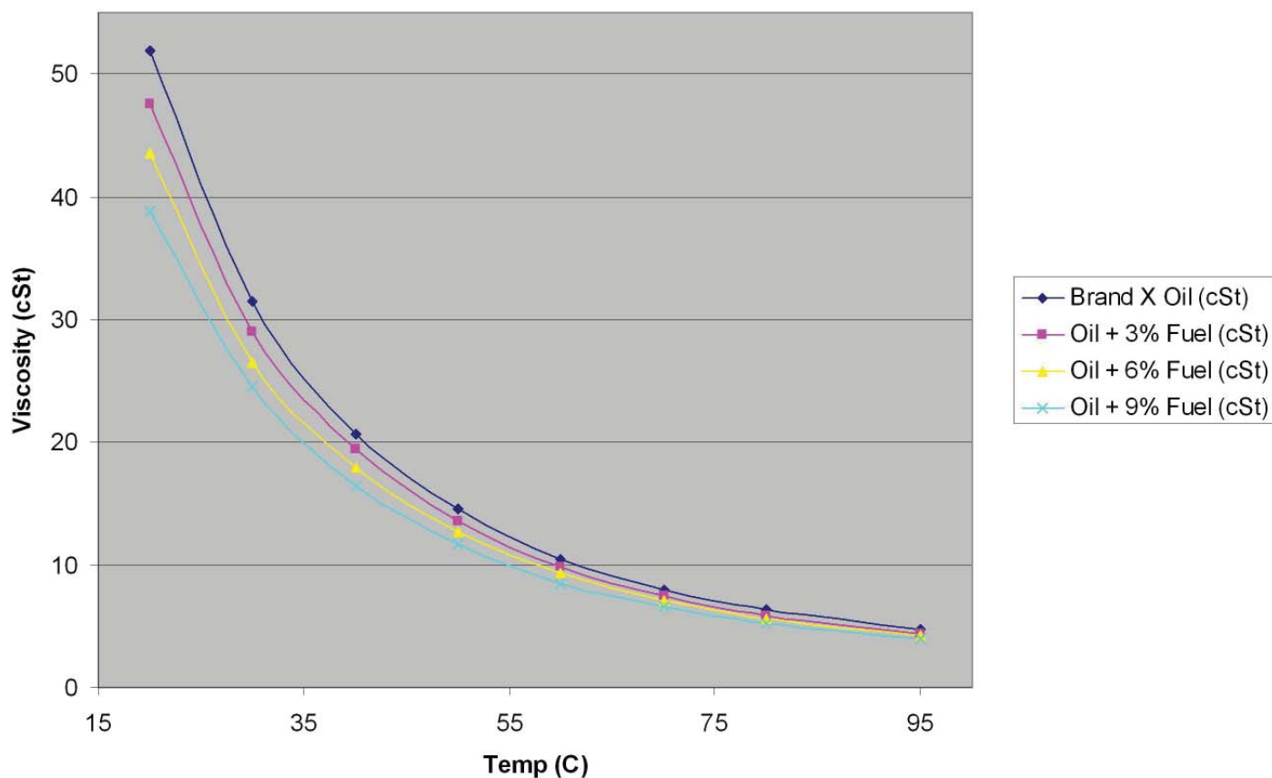
Figure 1: Viscosity changes as a function of fuel dilution across a temperature range using the ViSmart
